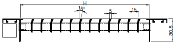
LM1 standard blade type
